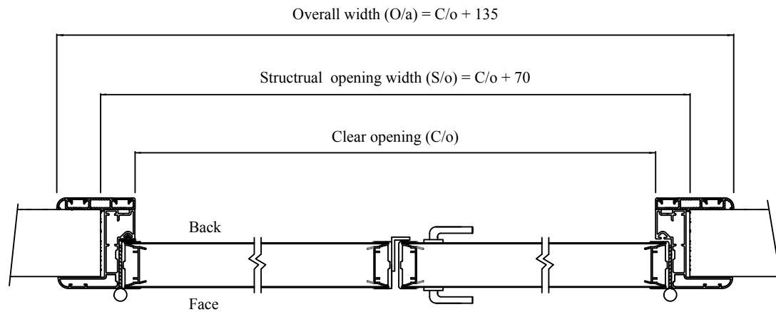
Horizontal section
