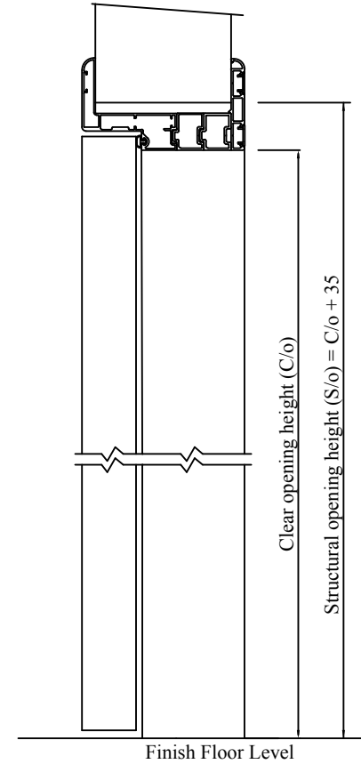
Vertical section
